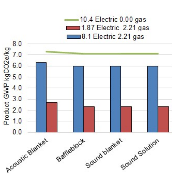
Figure 5. PET Fibre GWP kg CO 2e /kg
