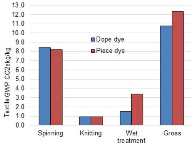
Figure 6. PET Fabric GWP kg CO 2e /kg
